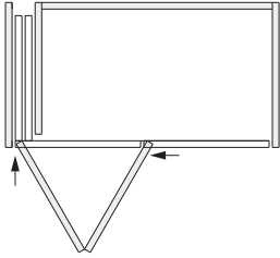
Hawa Folding Concepta III 25 Push, 左, 氧化铝
