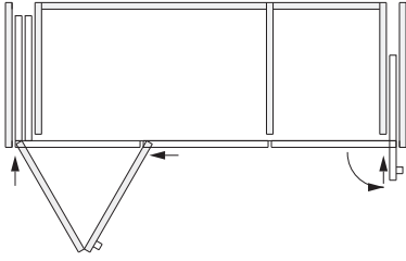
Hawa Folding Concepta III 20 Pull, 左, Hawa Concepta III 25 Pull, 右, 氧化铝
