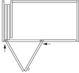
Hawa Folding Concepta III 20 Pull, 左, 氧化铝
