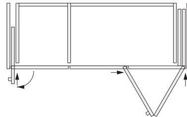
Hawa Folding Concepta III 25 Pull, 右, Hawa Concepta III 35 Pull, 左, 氧化铝
