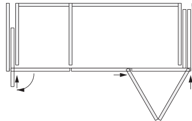
Hawa Folding Concepta III 20 Push, 右, Hawa Concepta III 25 Push, 左, 氧化铝
