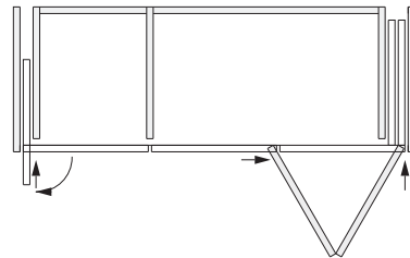
Hawa Folding Concepta III 25 Push, 右, Hawa Concepta III 35 Push, 左, 氧化铝
