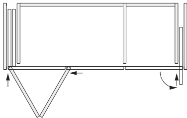
Hawa Folding Concepta III 20 Push, 左, Hawa Concepta III 25 Push, 右, 氧化铝
