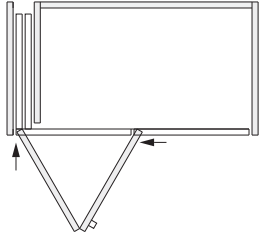
Hawa Folding Concepta III 25 Pull, 左, 氧化铝
