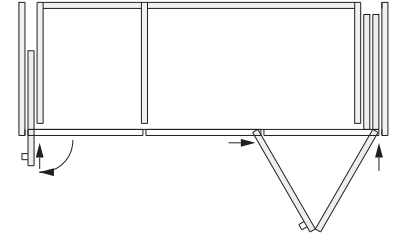
Hawa Folding Concepta III 20 Pull, 右, Hawa Concepta III 25 Pull, 左, 氧化铝
