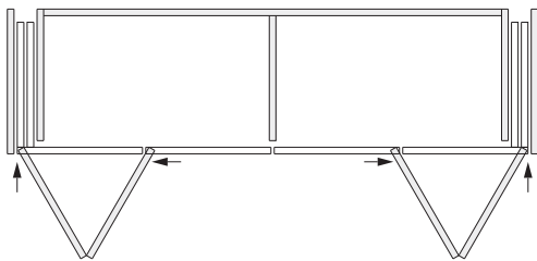
Hawa Folding Concepta III 20 Push, 左/右, 氧化铝
